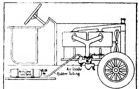
Fig. 2.—Emergency use of acetylene gas to run motor when gasoline supply is exhausted
